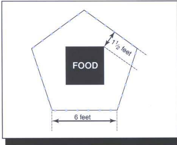
Figure 4—A recommended fence enclosure for backpacker's food would have five 6-foot-long sides. Food must be stored at least 1½ feet away from the fence. Outfitters needing to protect more food can combine two of these fences to enclose an area with 12-foot-long sides.
