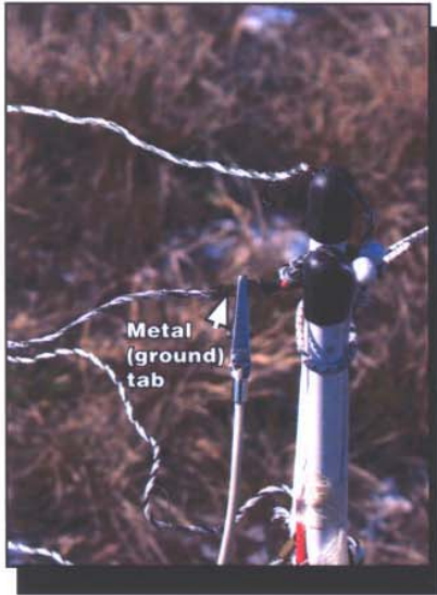
Figure 10—Clip the leads from the energizer to the hot wire (shown) and ground wires of the fence.
