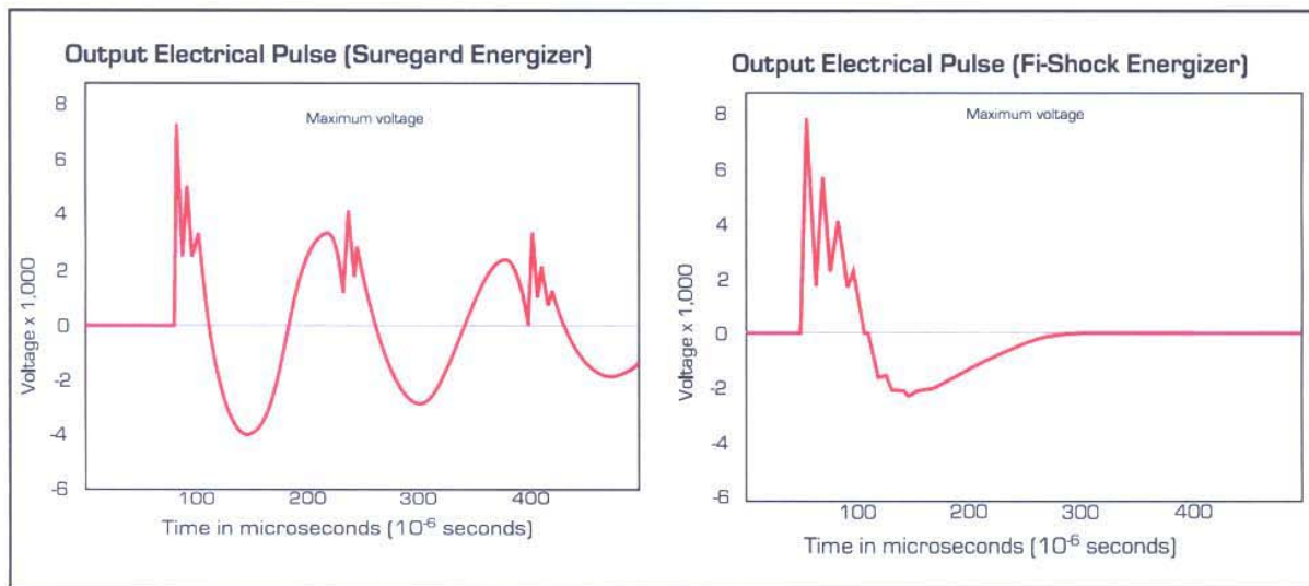
Figure 2—Different energizers have different pulse shapes. Effectiveness appears to be a factor of the total area (shaded) under the waveform curve. The “ringing” or oscillating pulse on the left appears to be more effective than the pulse on the right. Also, a pulse with higher voltage and amperage but a short duration is more effective and safer than a lower voltage with a longer duration.
