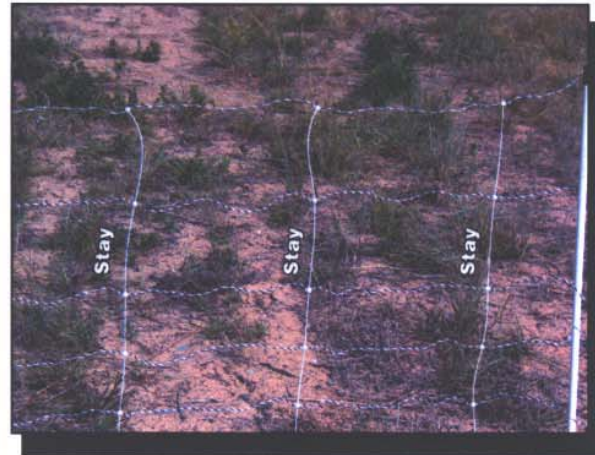
Figure 3a—Semirigid vertical stays (above) are preferred to flexible vertical strands (figure 3b, below), because they prevent hot wires from sagging and shorting out the fence.
