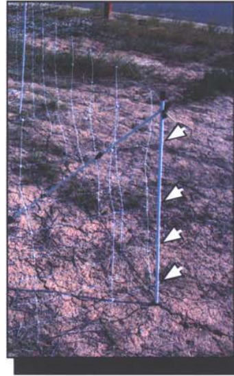
Figure 8—Make sure that the hot wires (arrows) are on the outside of the fence posts. Otherwise, a bear could knock the post over without getting shocked.
